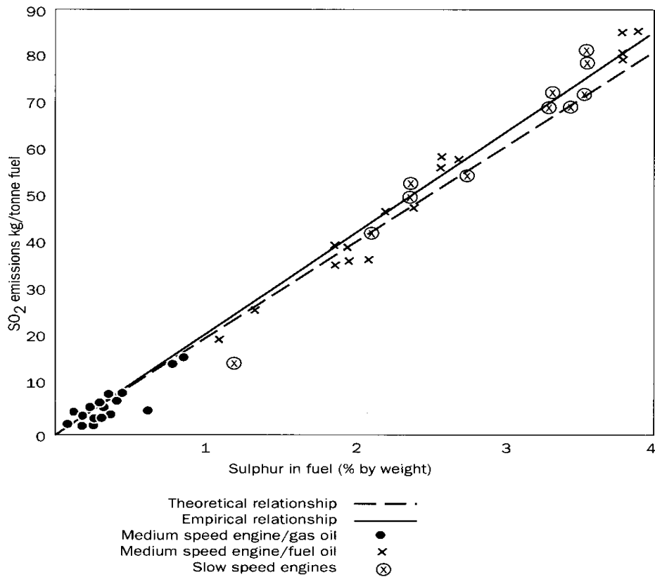
Figure 3 Relationship between fuel sulphur content and SO 2 emissions for marine diesel engines (Lloyds Register 1995)
