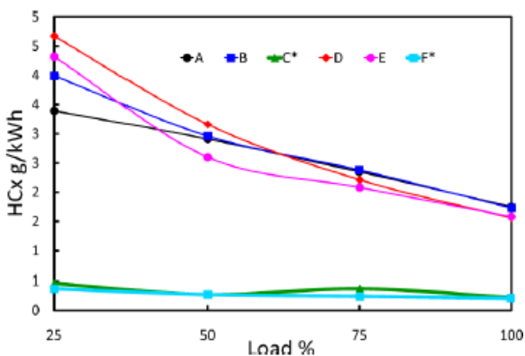
Figure 8 HC emissions for 2 stroke engines (C* and F* fulfil Tier II NOx levels, CIMAC 2010)
