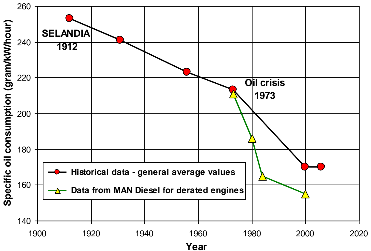
Figure 1 Development of specific oil consumption for two stroke slow speed diesel engines (test bed conditions, 42.7 MJ/kg oil)
