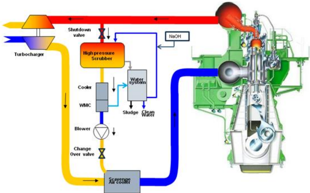
Figure 6 Principles of an EGR system (MAN Diesel)
