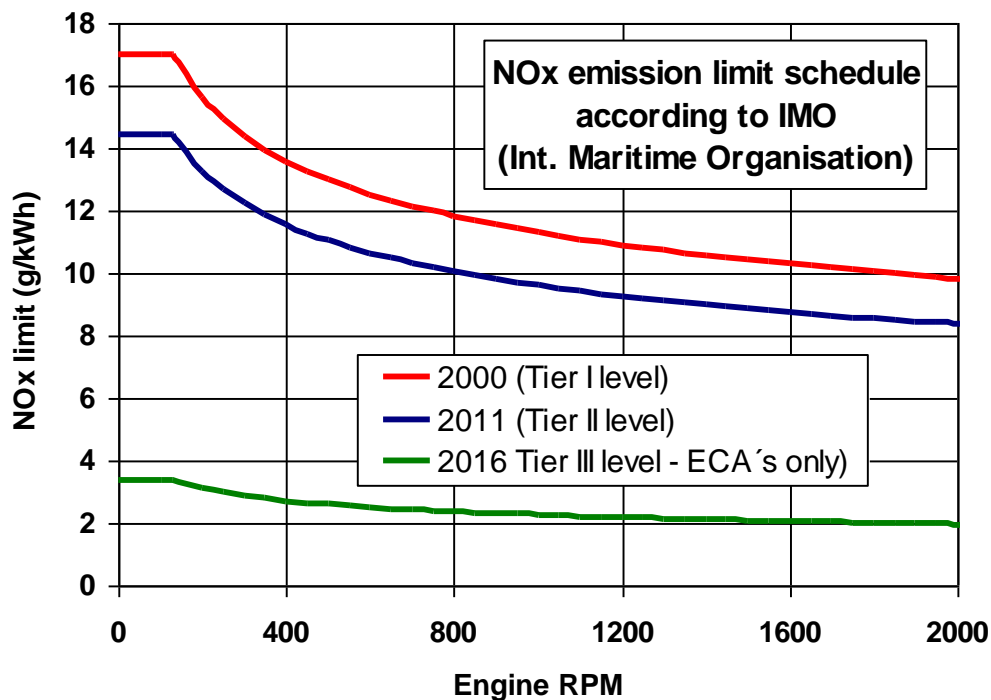
Figure 5 Maximum allowable fuel specific NOx emission rate according to IMO, MARPOL Annex VI
