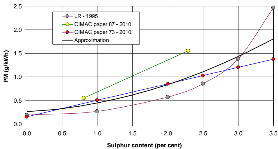
Fig. 7 Relationship between fuel sulphur content and emissions of particulates, PM (Lloyds Register 1995 and CIMAC 2010)
